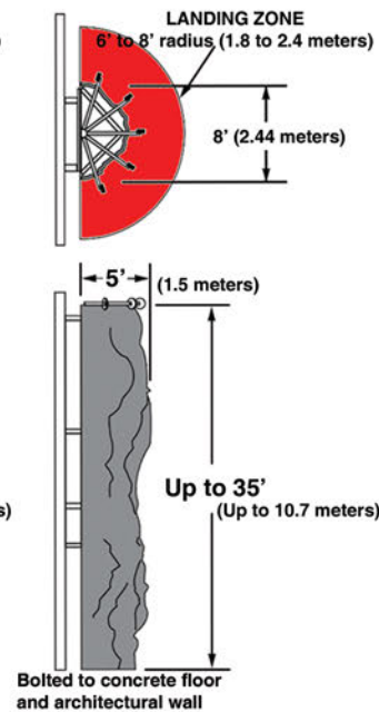
Typical Flush Mount 1/2 Tower
