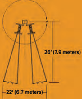
TANDEM JUMPER CONFIGURATION
